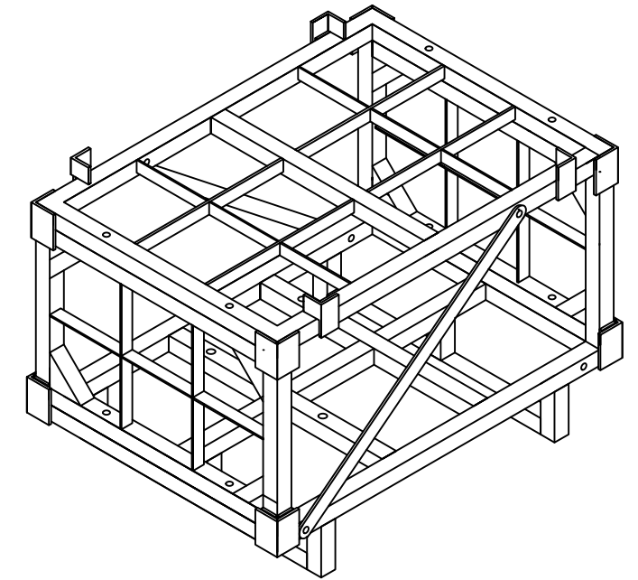
Complete Box Assembly Isometric View
