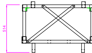
Frame in Assembled Condition
